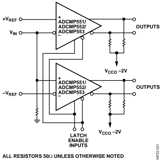
ALL RESISTORS 50Ω UNLESS OTHERWISE NOTED Figure 22. High Speed Window Comparator
