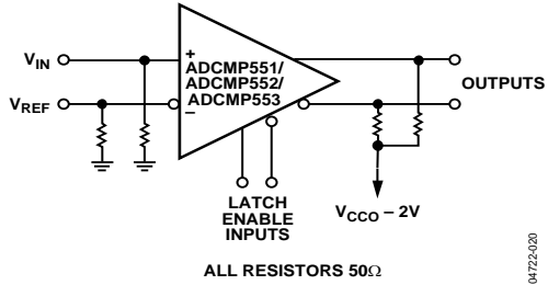
ALL RESISTORS 50Ω Figure 21. High Speed Sampling Circuits
