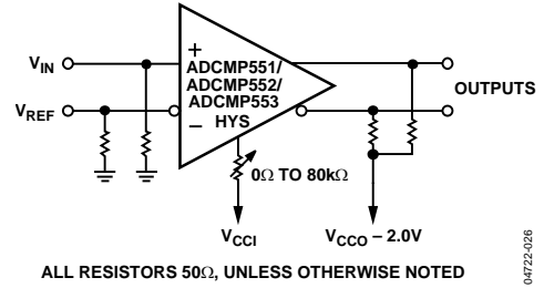
ALL RESISTORS 50Ω, UNLESS OTHERWISE NOTED Figure 23. Adding Hysteresis Using the HYS Control Pin
