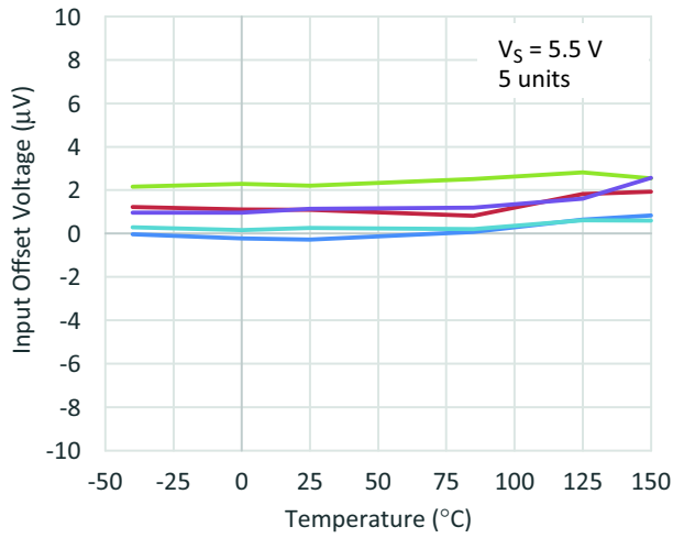
Figure 5. Input Offset Voltage vs. Temperature at 5.5 V Supply
