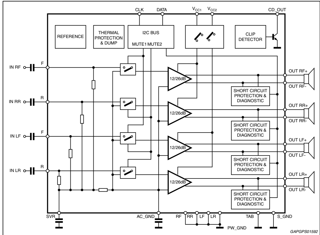
Figure 1. Block diagram
