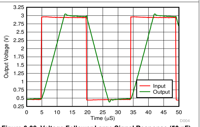
Figure 6-38. Voltage Follower Large Signal Response (50 pF)
