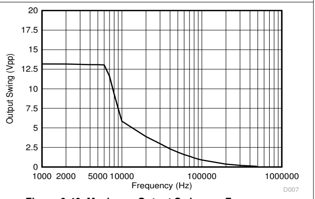
Figure 6-40. Maximum Output Swing vs. Frequency (VCC = 15 V)
